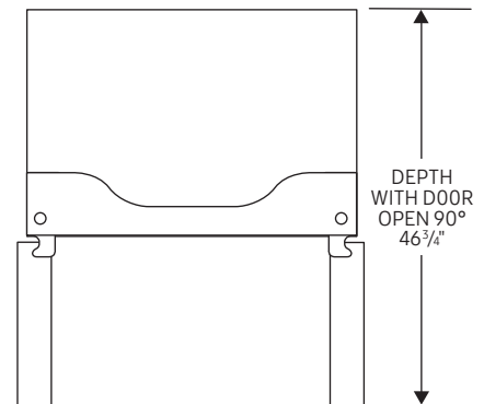
TOP OF REFRIGERATOR WITH DOOR OPEN 90°
