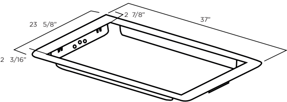
TRIM KIT DIMENSIONS
