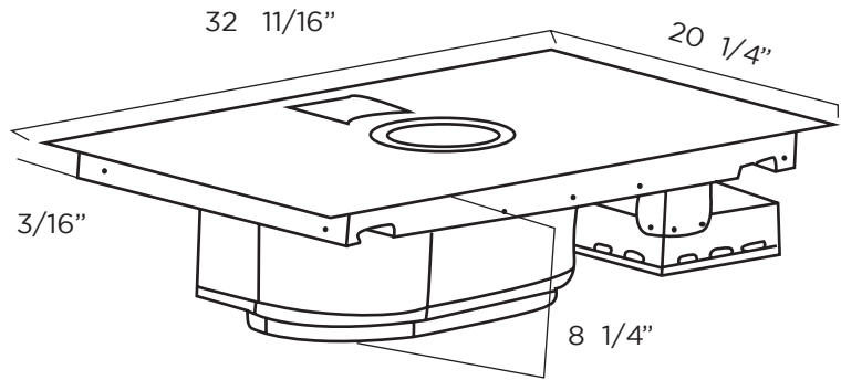
TRIM KIT DIMENSIONS
