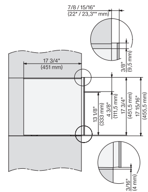
CVA7440, CVA7840, side view, 60 cm, Proud
